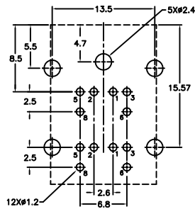
P.C. Board Layout (Top View)
